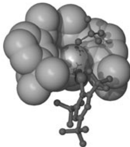
Fig. 1. Using steric bulk to protect a rare Ti=P bond.
