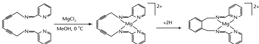
Fig. 4. Cyclizing a magnesium-complexed "ene-diyne" damages DNA by double H-atom abstraction.
