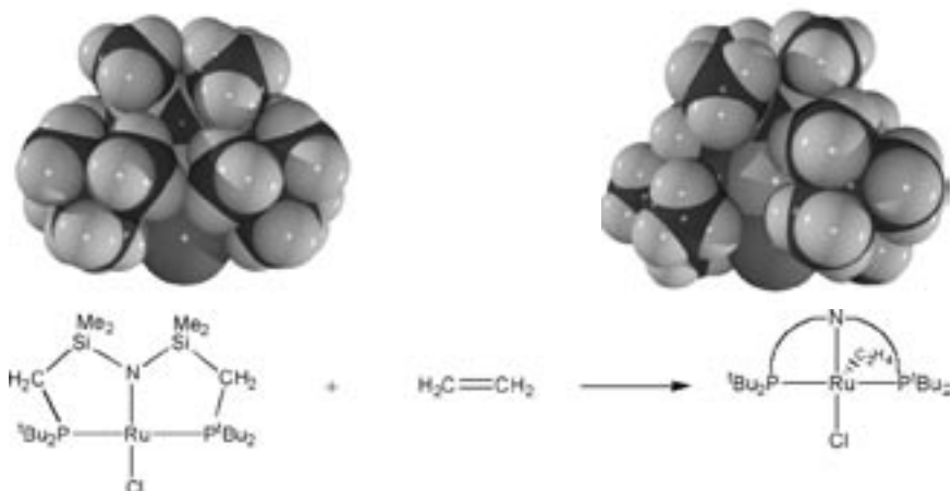
Fig. 5. Arriving C_2H_4 molecule sterically shields the ruthenium atom by distorting the tBu groups.
